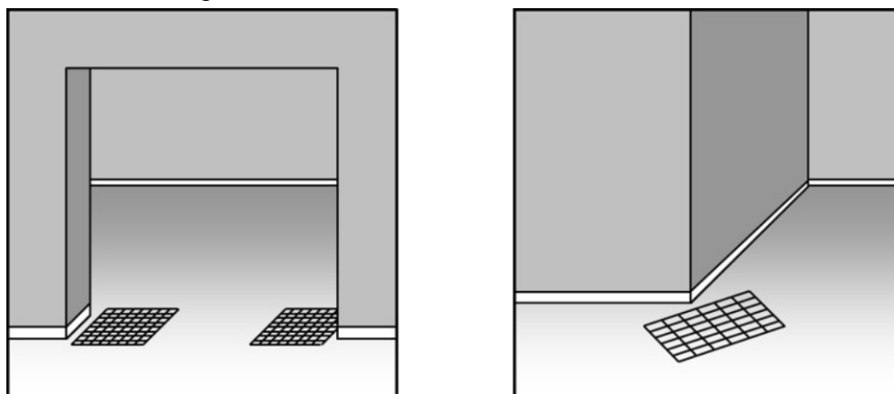
Figure 1 – Renforts d'angle
